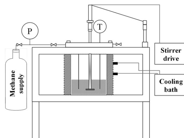
Fig. 1 – Structure of the methane hydrate formation apparatus.
