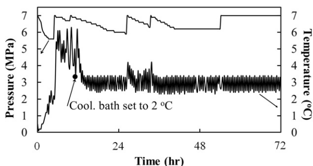
Fig. 2 – Pressure and temperature for methane hydrate formation.
